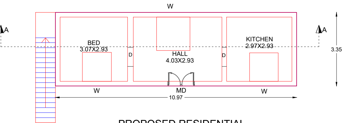
PROPOSED RESIDENTIAL GROUND FLOOR PLAN
