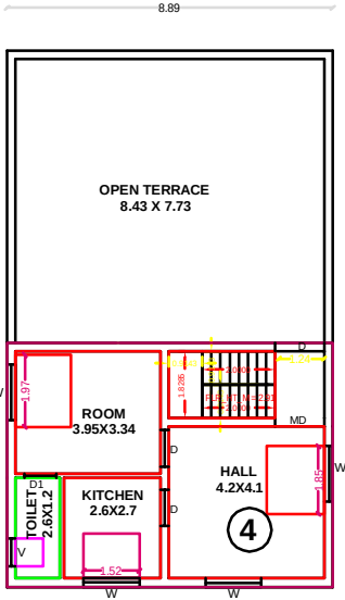
SECOND FLOOR PLAN PROPOSED
