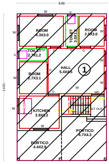
GROUND FLOOR PLAN EXISTING
