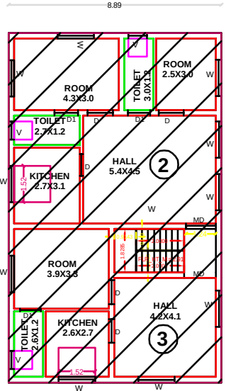
FIRST FLOOR PLAN EXISTING
