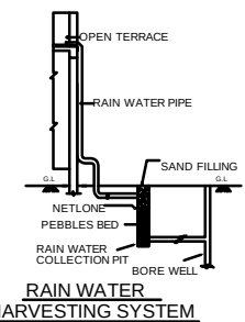
RAIN WATER HARVESTING SYSTEM
