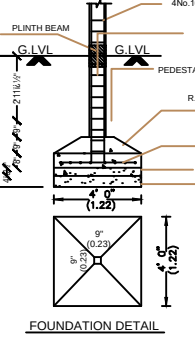
FOUNDATION DETAIL
