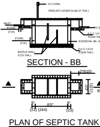
PLAN OF SEPTIC TANK
