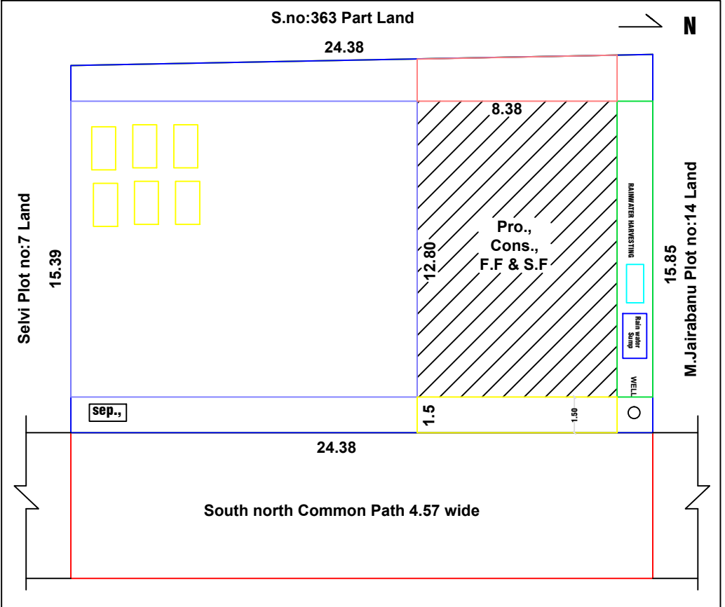
SITE PLAN CUM KEYPLAN
