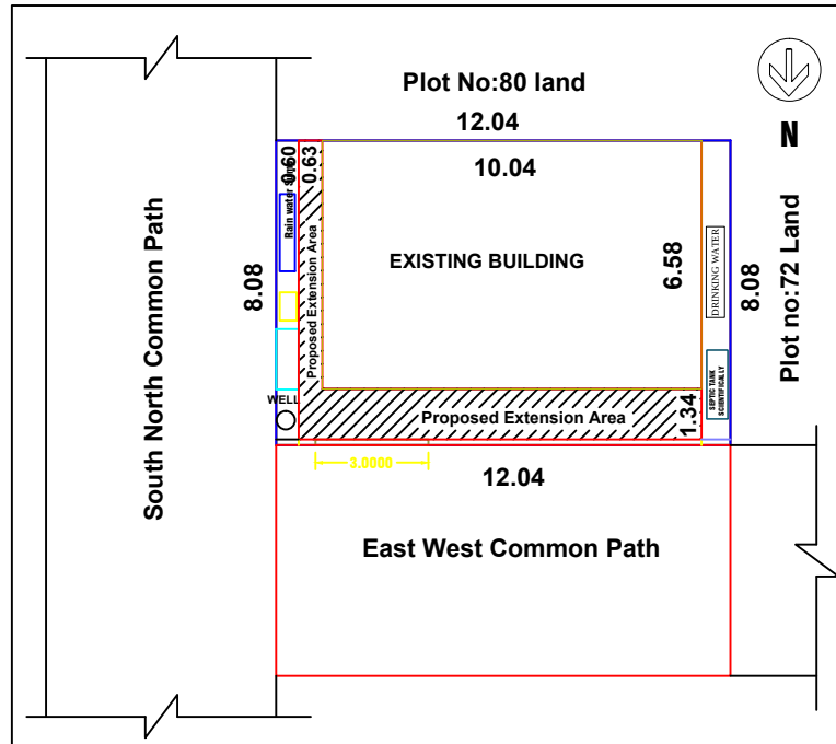
SITE PLAN & KEY PLAN
