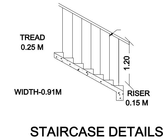
STAIRCASE DETAILS
