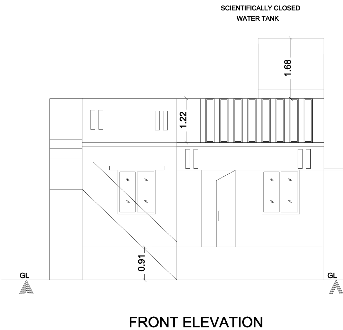
FRONT ELEVATION
