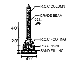
COLOUMN FOUNDATION
