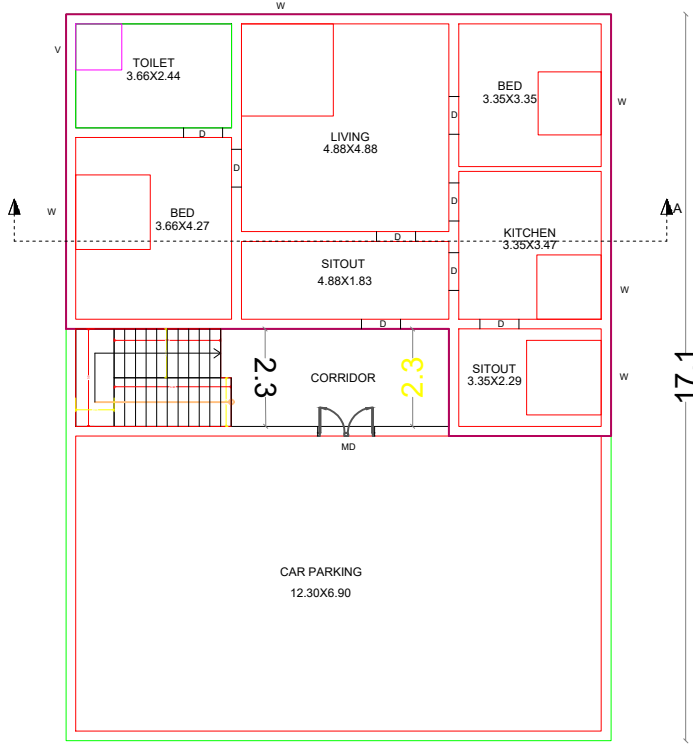
PROPOSED RESIDENTIAL FIRST FLOOR PLAN
