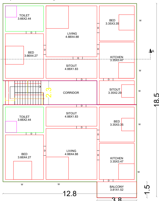
PROPOSED RESIDENTIAL SECOND FLOOR PLAN
