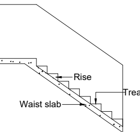
DETAIL OF STAIRCASE
