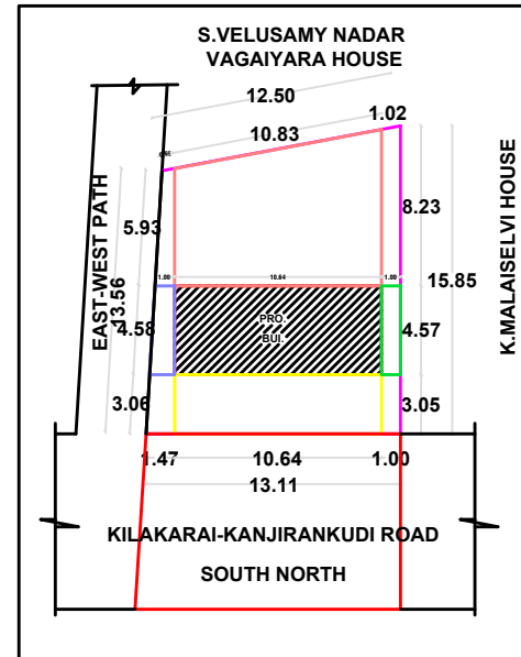
SITE PLAN & KEY PLAN
