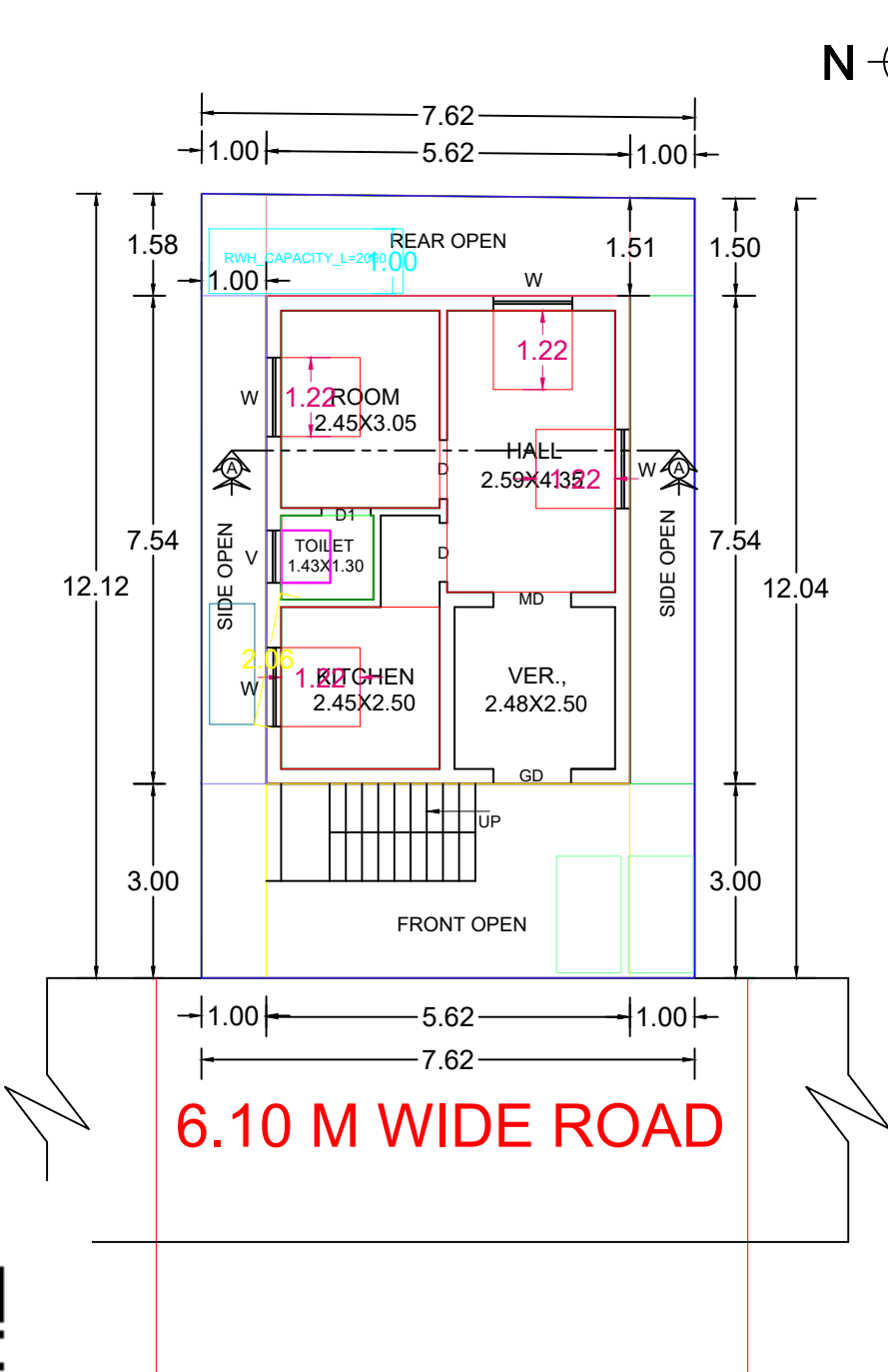
SITE PLAN CUM GROUND FLOOR PLAN
