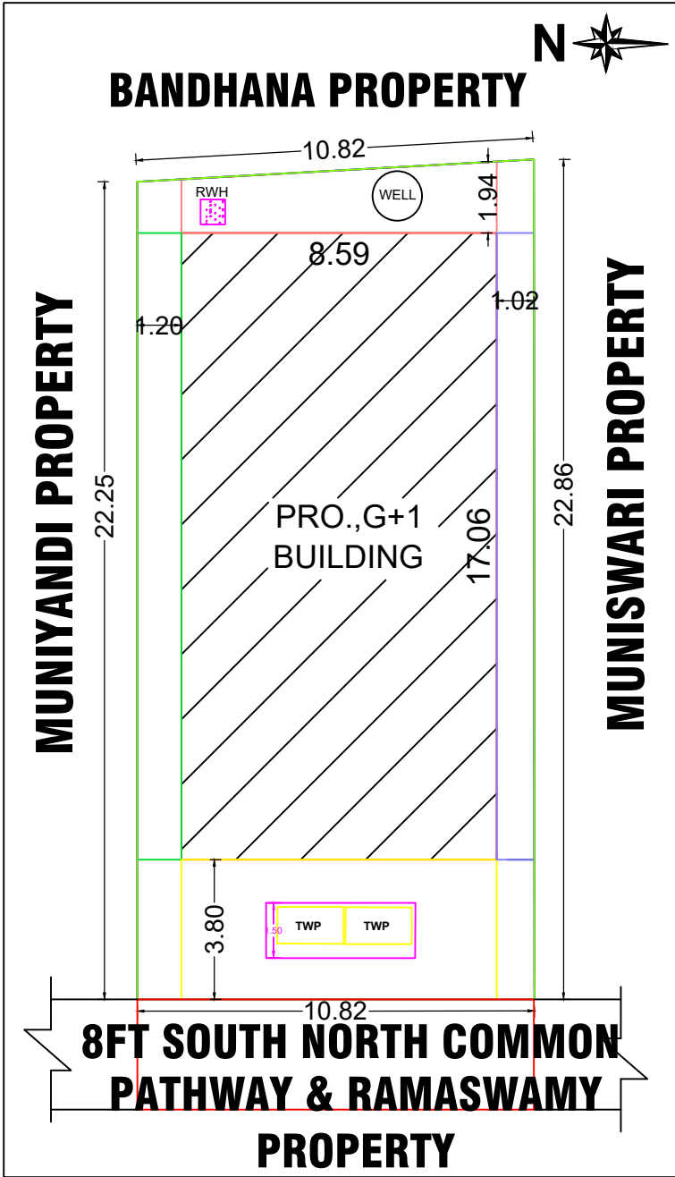
SITE PLAN
