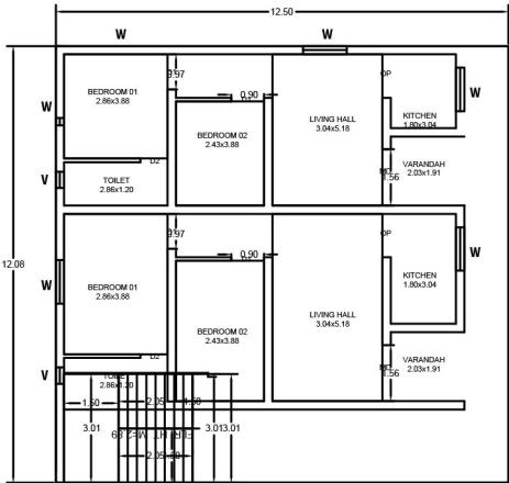
PRO., FIRST FLOOR PLAN
