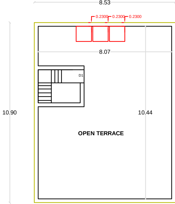
TERRACE FLOOR PLAN PROPOSED
