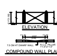
COMPOUND WALL PLAN
