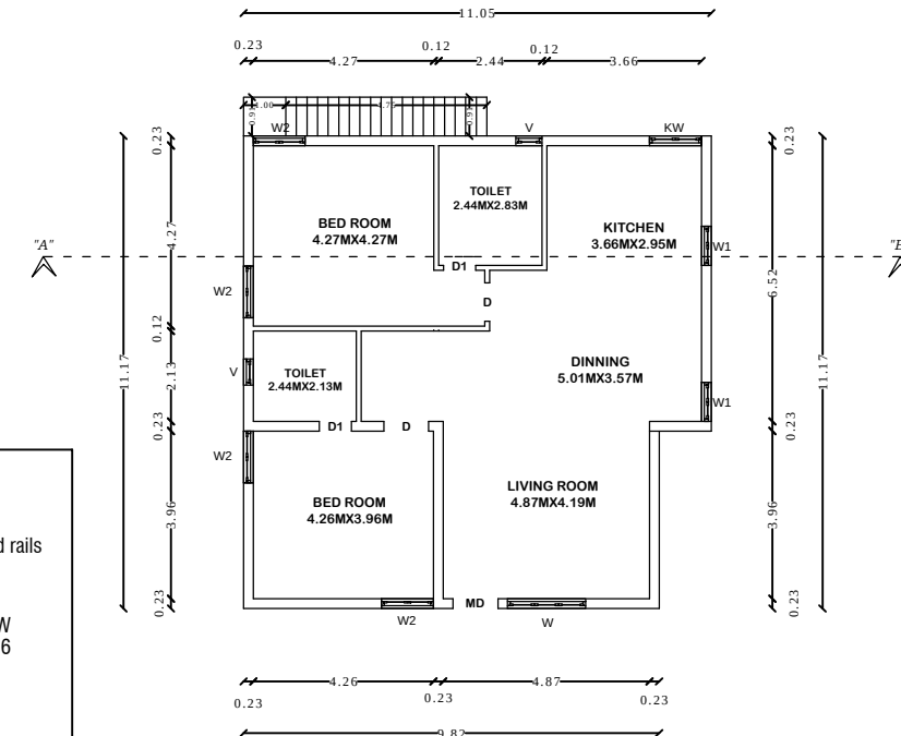
PROPOSED GROUND FLOOR PLAN SCALE - 1":8'0"[1:100] RESIDENTIAL BUILDING
