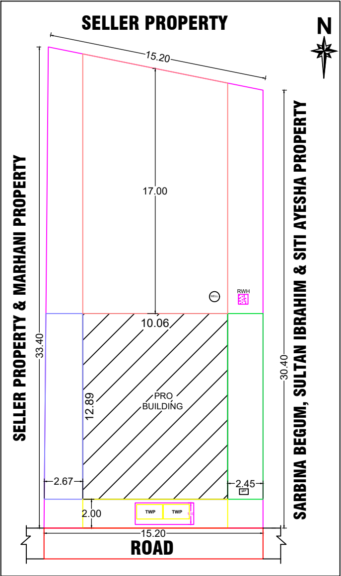
SITE PLAN
