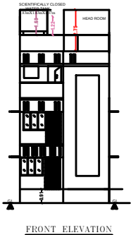
FRONT ELEVATION
