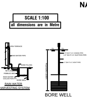
BORE WELL
