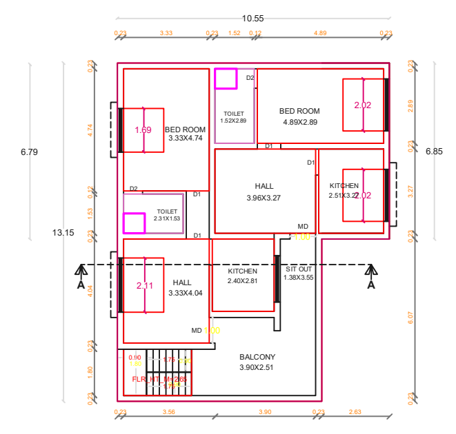
FIRST FLOOR PLAN PROPOSED
