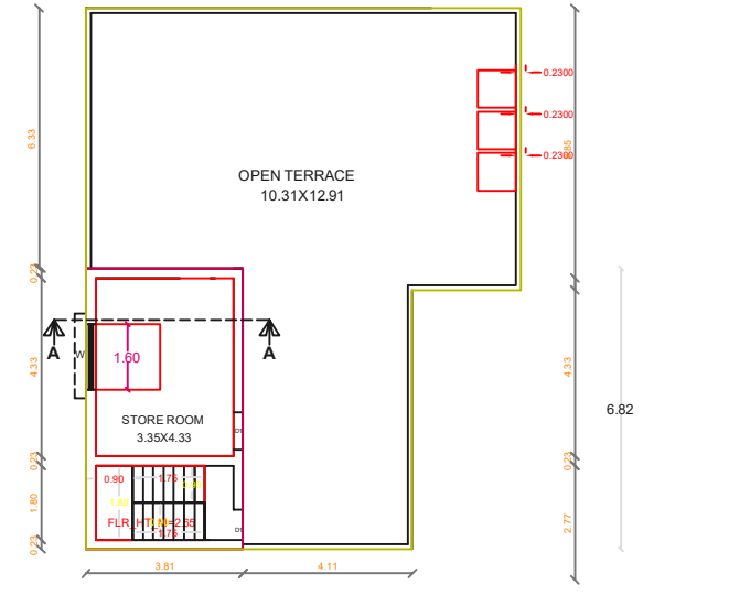
SECOND & TERRACE FLOOR PLAN PROPOSED
