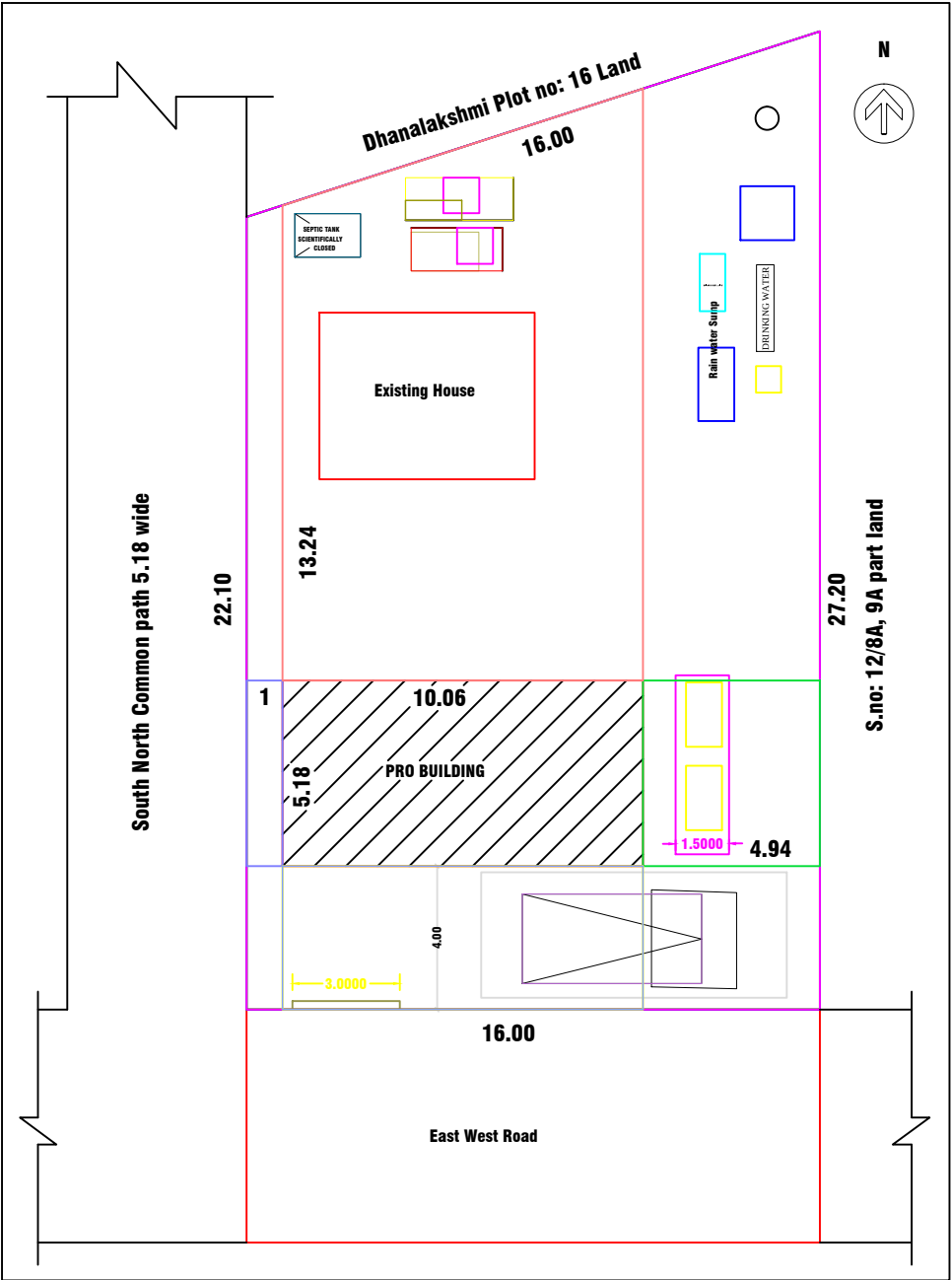
SITE PLAN & KEY PLAN
