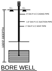
BORE WELL
