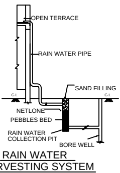
RAIN WATER HARVESTING SYSTEM
