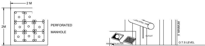
PLAN OF RAIN WATER RECHARGING PIT
