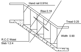
STAIRCASE DETAIL
