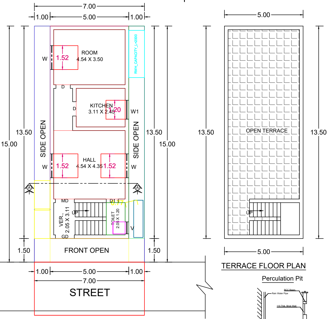
SITE PLAN CUM GROUND FLOOR PLAN
