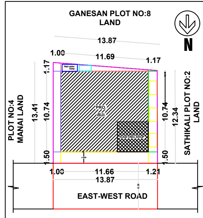
SITE PLAN & KEY PLAN
