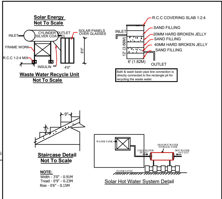
PERCOLATION PIT
