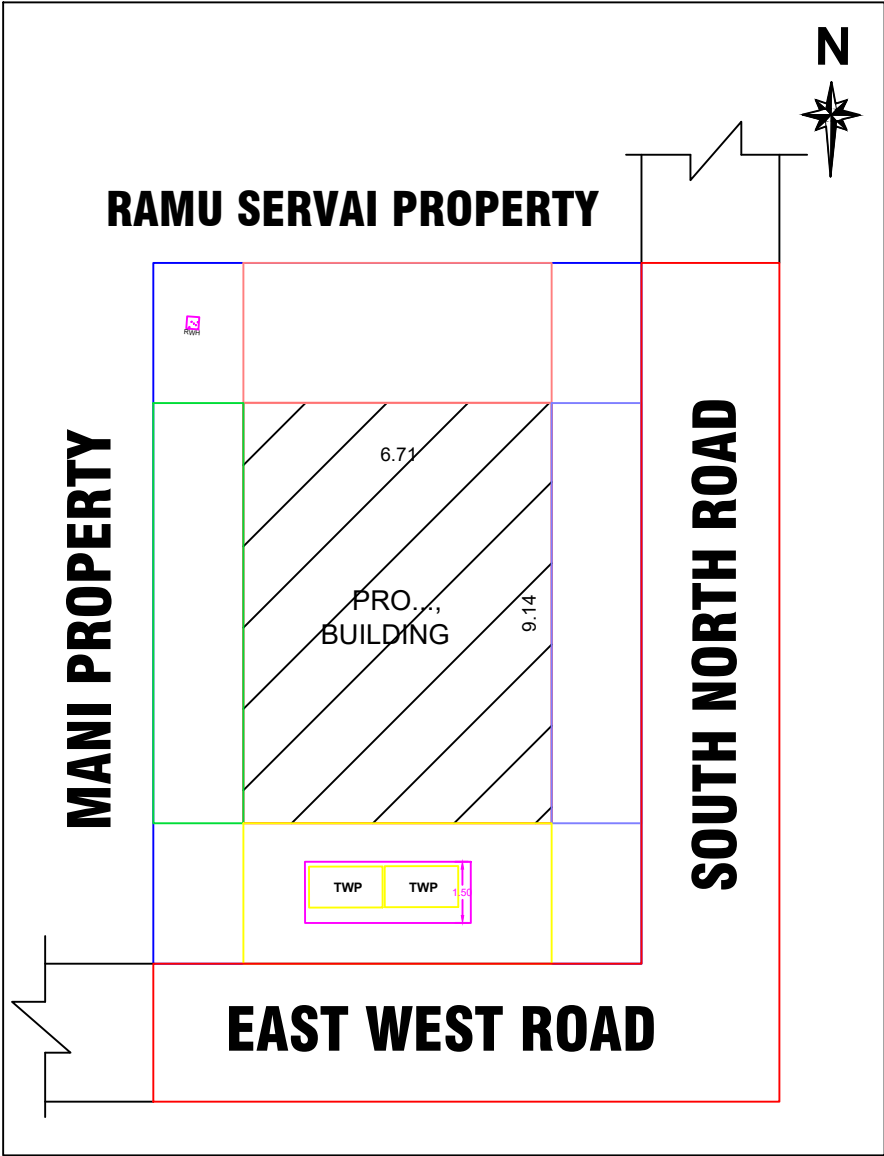
SITE PLAN
