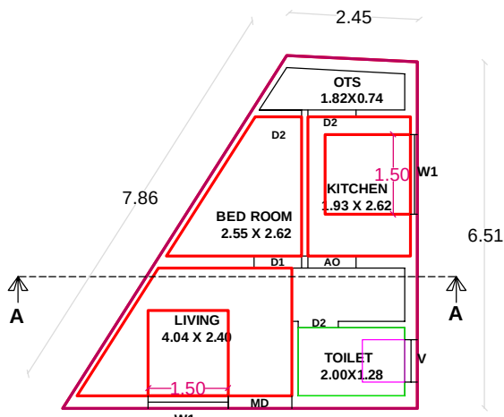
GROUND FLOOR PLAN PROPOSED
