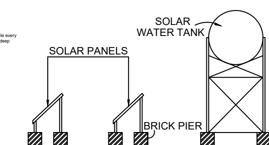
SECTION OF SOLAR HEATER
