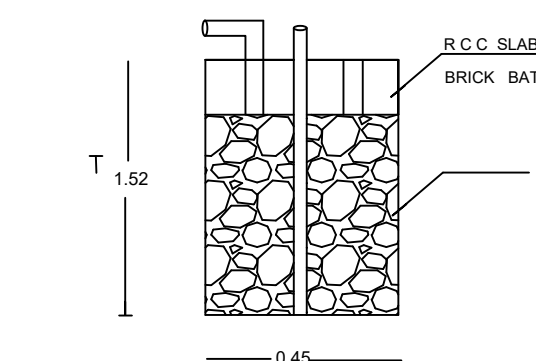
RAIN WATER STORAGE
