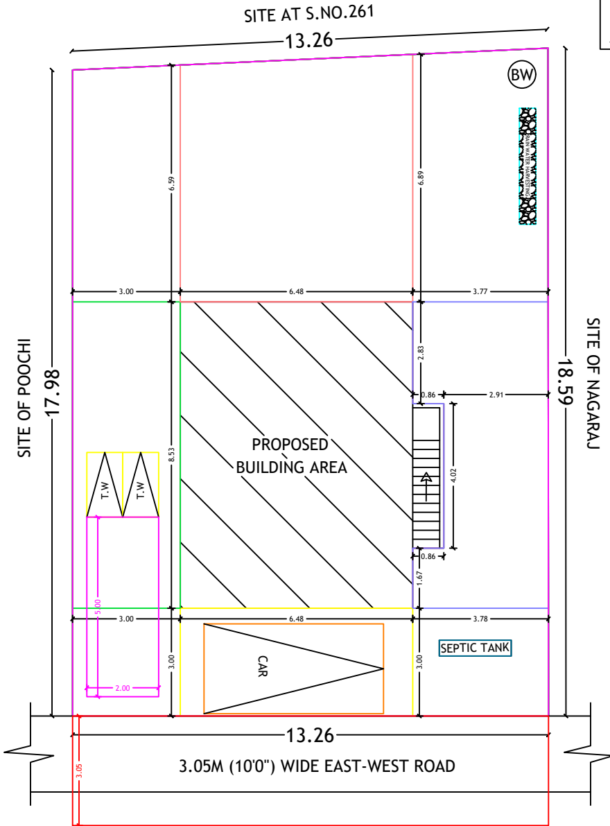
SITE PLAN
