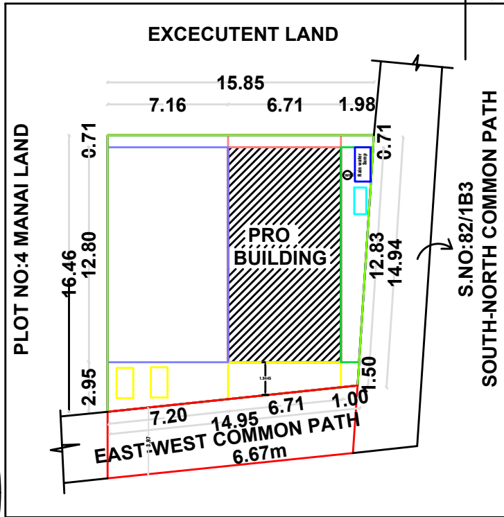
SITE PLAN & KEY PLAN (1:100)
