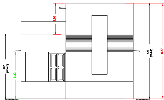
ELEVATION-B
