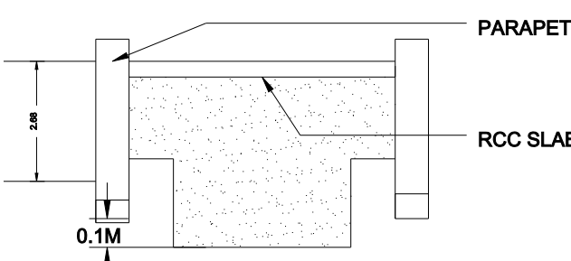
SECTION
