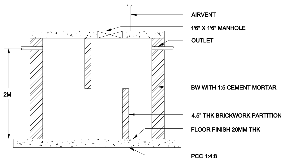
CROSS SECTION OF SEPTIC TANK
