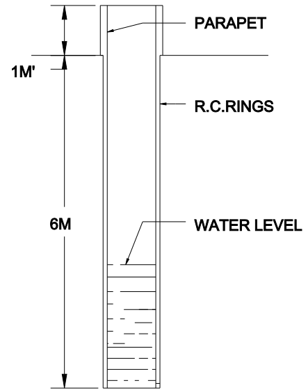
C.S OF WELL
