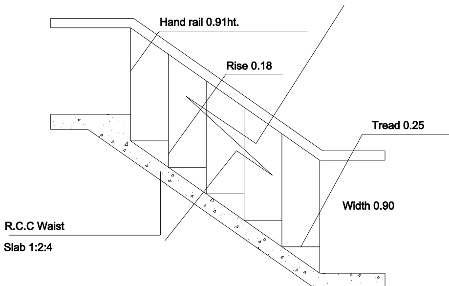
STAIRCASE DETAIL
