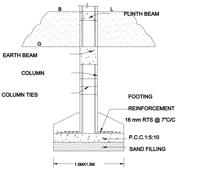
FOUNDATION DETAIL
