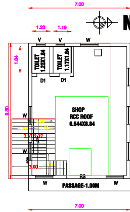
EXI-FIRST FLOOR PLAN
