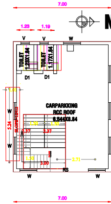
EXI-SILT FLOOR PLAN
