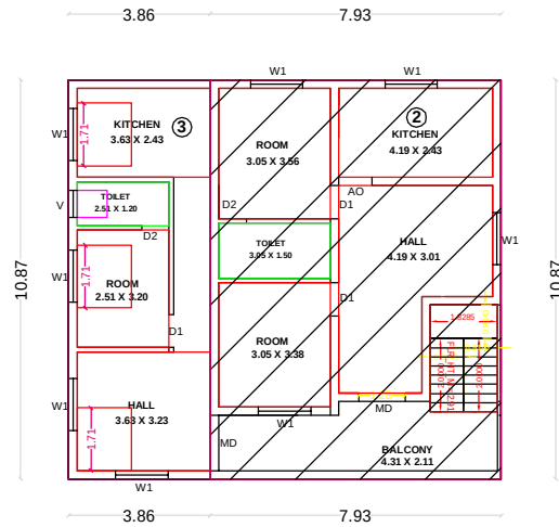
FIRST FLOOR PLAN EXISTING & PROPOSED
