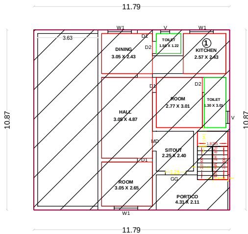
GROUND FLOOR PLAN EXISTING
