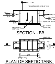
SECTION - BB PLAN OF SEPTIC TANK
