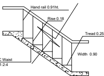
STAIRCASE DETAIL
