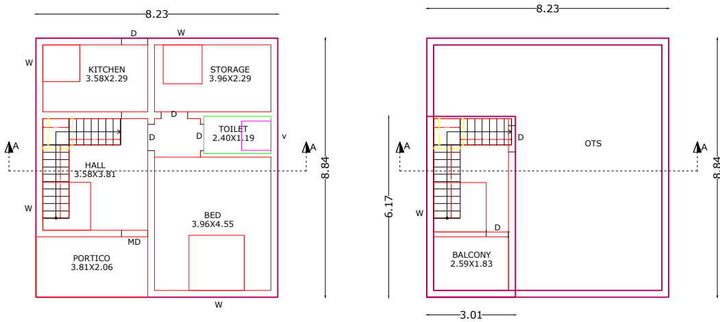
PROPOSED RESIDENTIAL GROUND FLOOR PLAN
