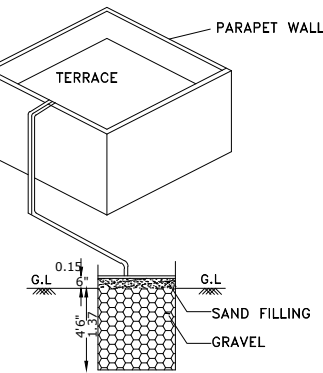
COLLECTION OF SUMP RAINWATER HARVESTING FROM TERRACE
