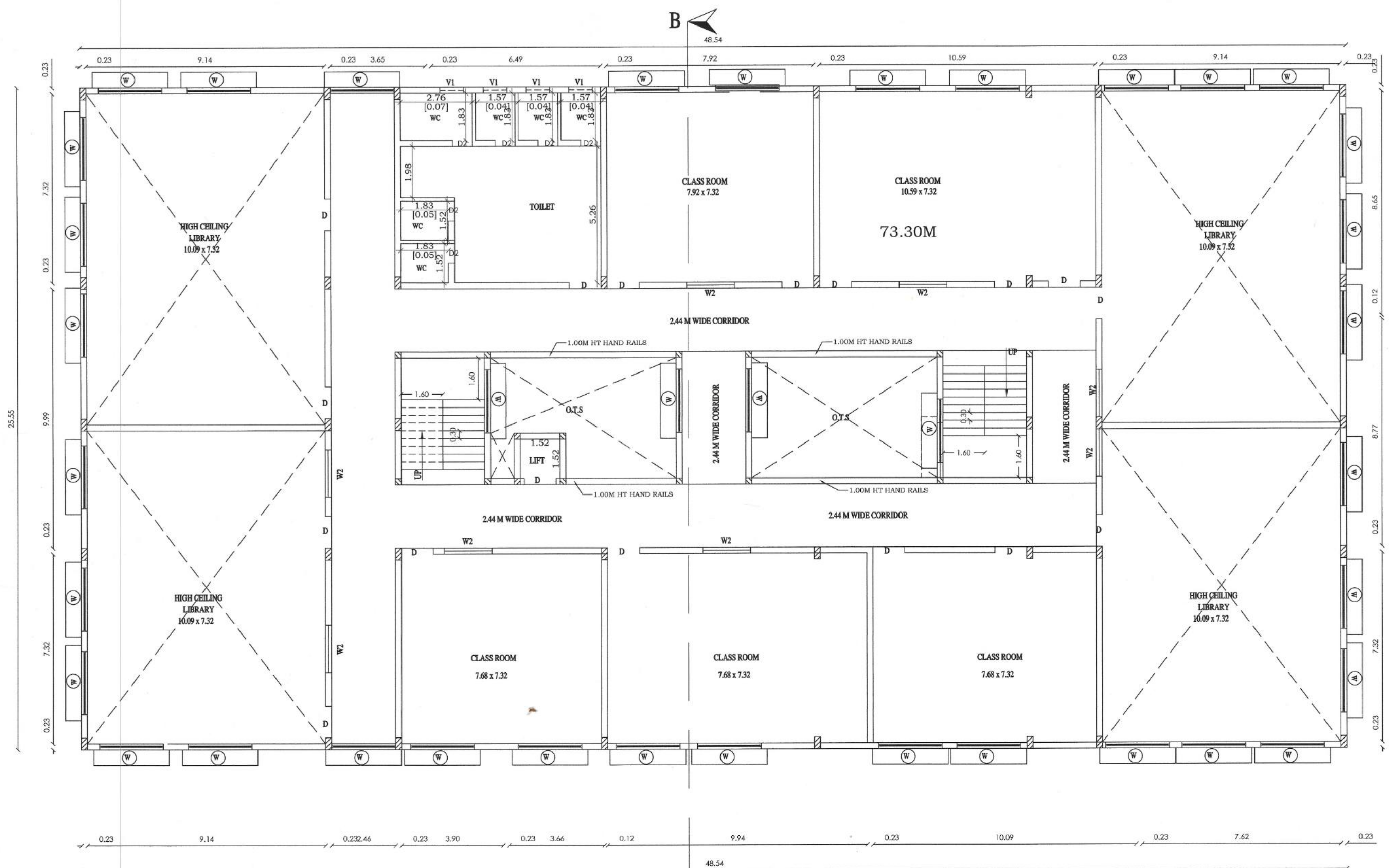
A PRO. SECOND FLOOR PLAN
