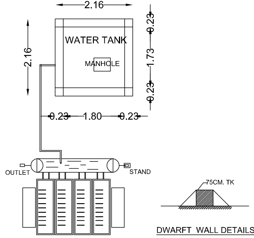
PLAN OF OHT SOLAR WATER HEATING SYSTEM
