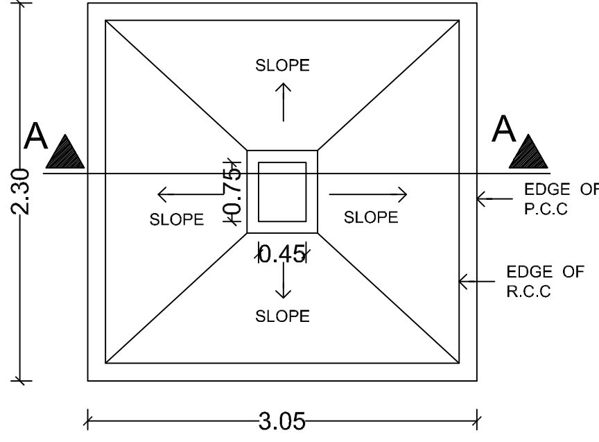
PLAN As per design Typical Column Foundation Detail As per design
