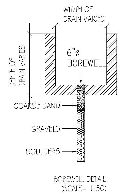
BOREWELL DETAIL (SCALE= 1:50)
