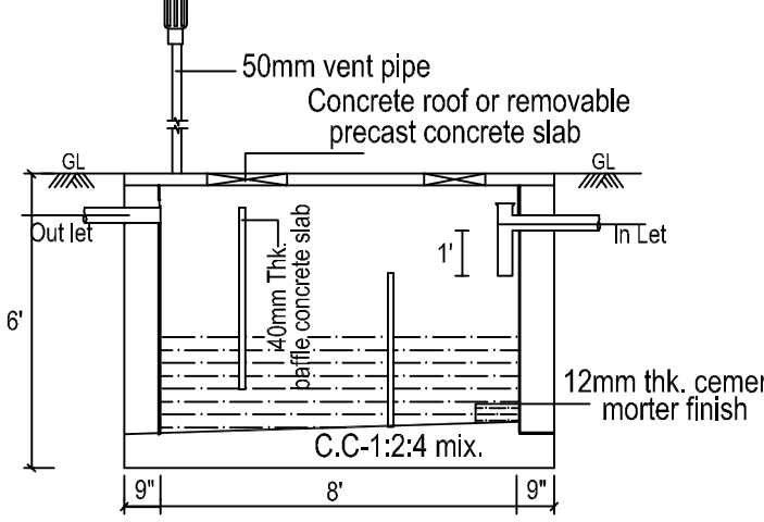
Sec. of Septic Tank
