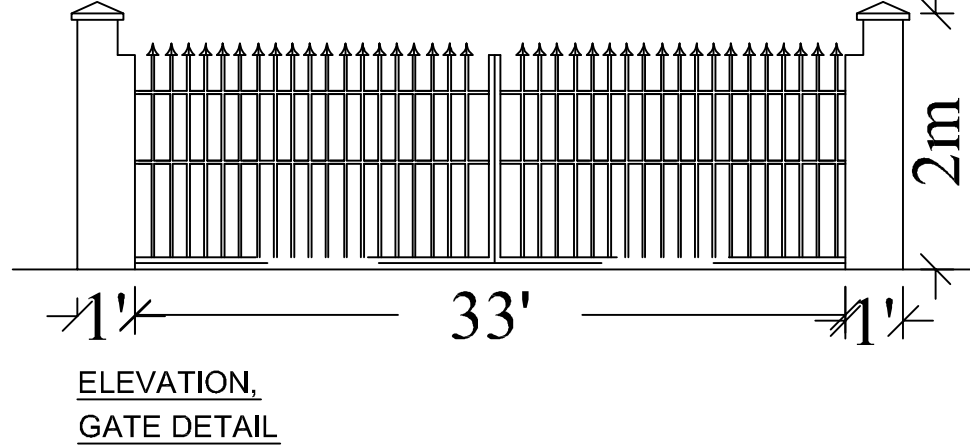
ELEVATION GATE DETAIL PLAN, GATE DETAIL
