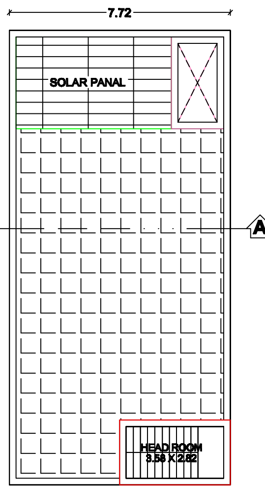
HEAD ROOM TERRACE FLOOR PLAN
