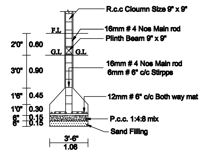
COLUMN DETIAL NOT TO SCALE
