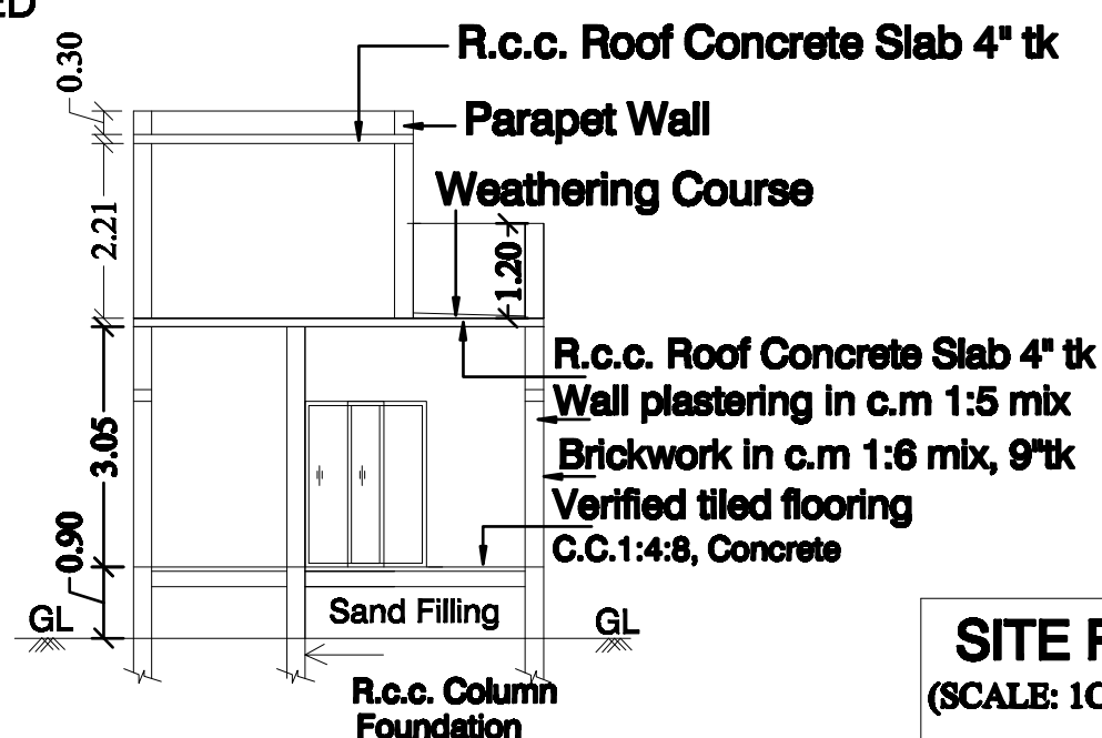
SECTION NN (SCALE: 1CM : 1M)
