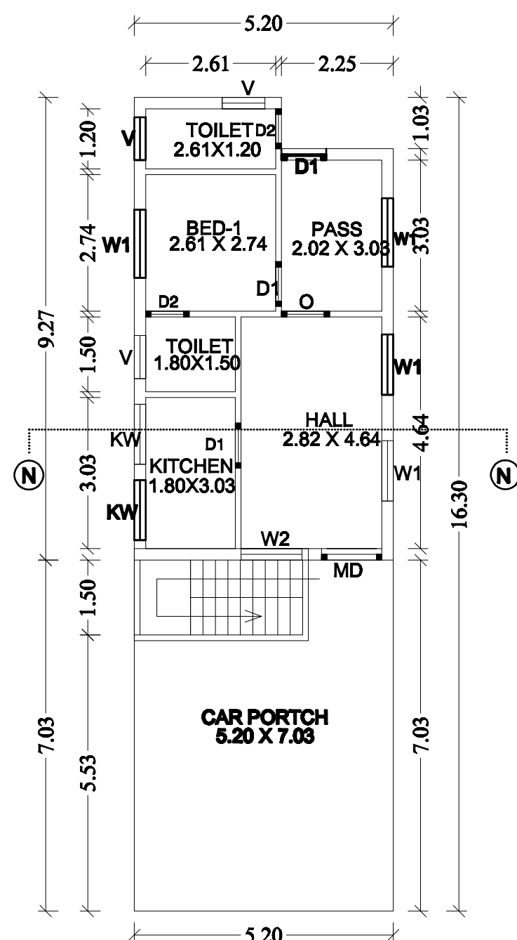
GROUND FLOOR AND HEAD ROOM PLAN
