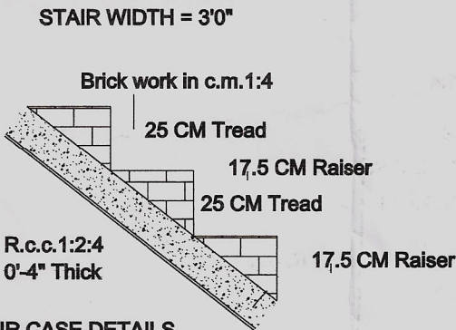
STAIR CASE DETAILS SCALE : 1" = 2'-0"
