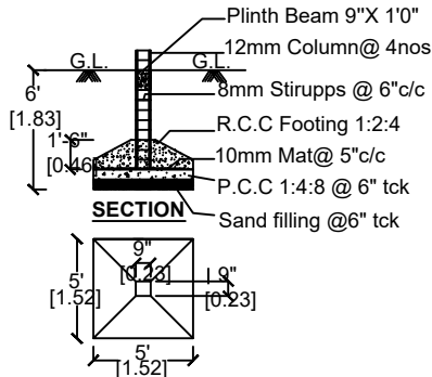
SIZE OF COLUMN 9"X9" COLUMN DETAIL
