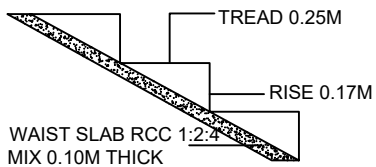
STAIR DETAILS
