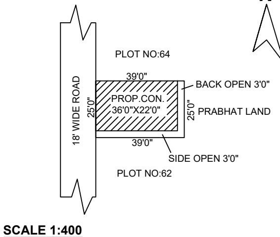
SITE PLAN
