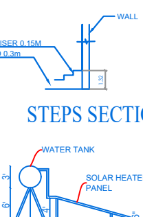
WATER TANK
