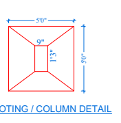
FOOTING / COLUMN DETAIL
