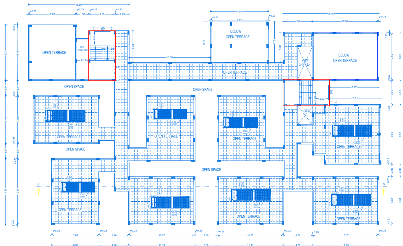
OPEN TERRACE FLOOR PLAN
