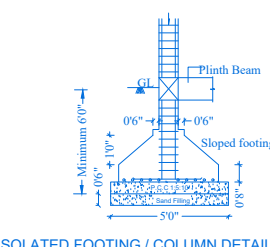
ISOLATED FOOTING / COLUMN DETAIL
