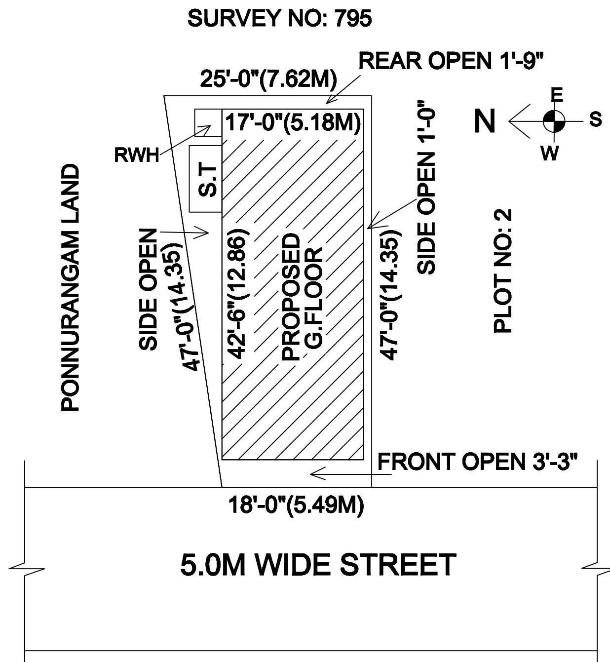
SITE PLAN
