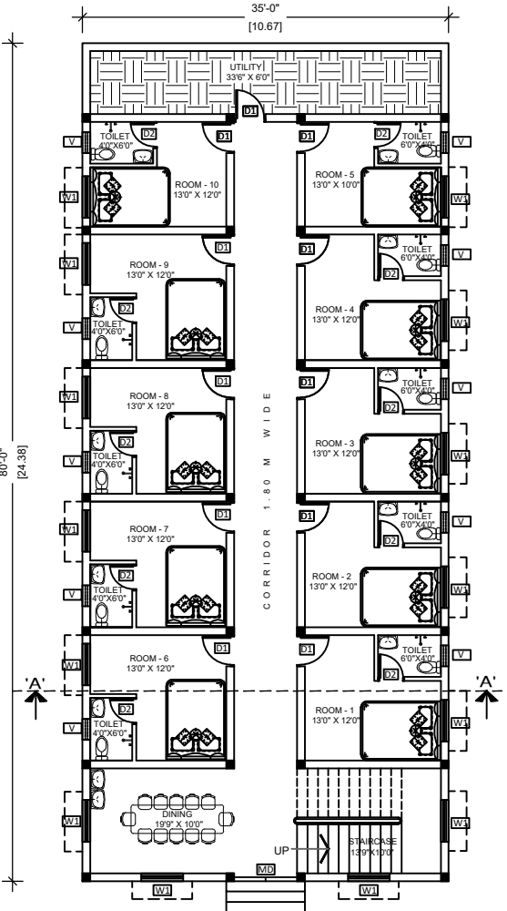
GROUND FLOOR PLAN ( BLOCK - II )
