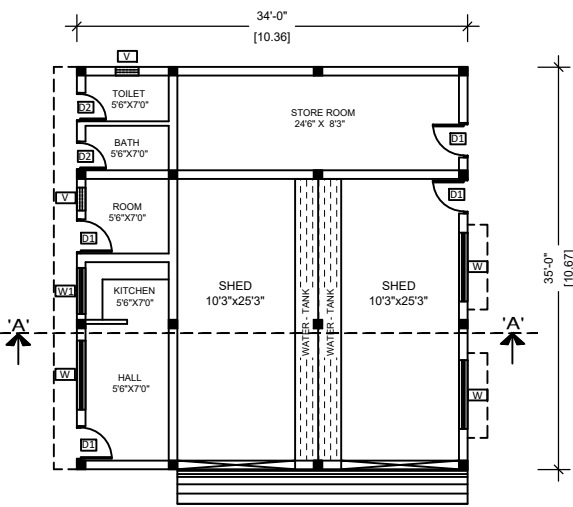
GROUND FLOOR PLAN ( BLOCK - I )
