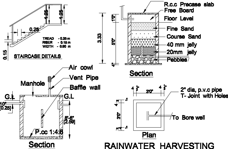
RAINWATER HARVESTING TANK SCALE 1:50
