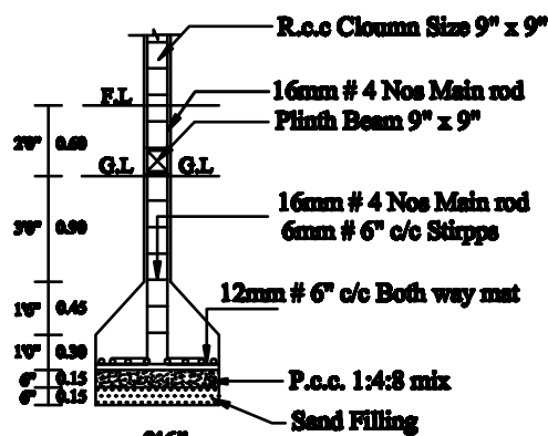
COLUMN DETIAL
