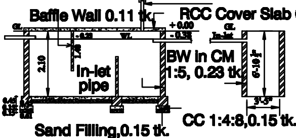
SEPTIC TANK & SOAK PIT
