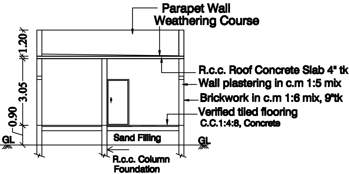
SECTION NN (SCALE: 1CM : 1M)
