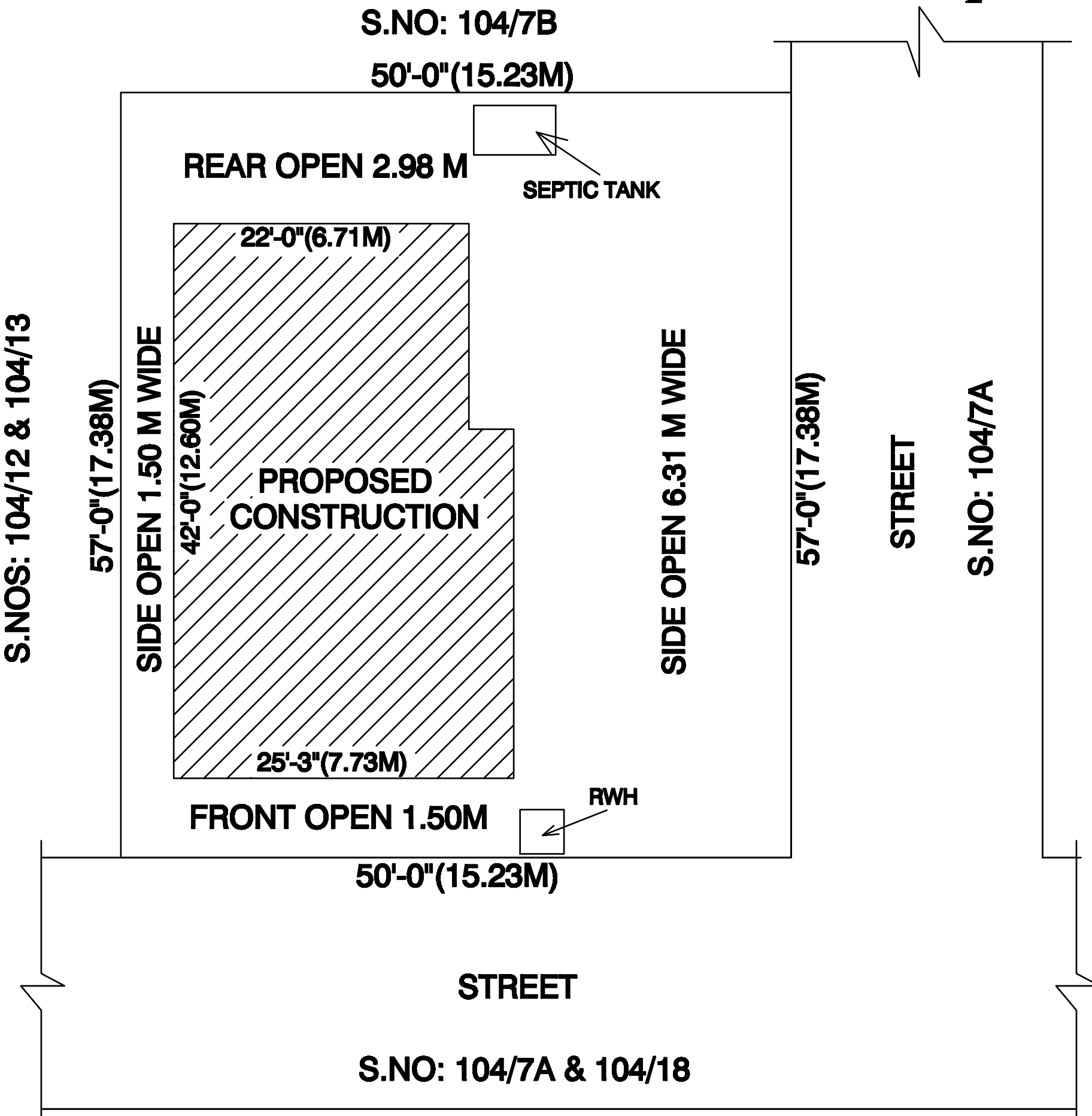
SITE PLAN (SCALE: 1CM : 1M)
