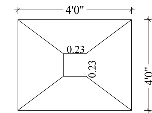
FOOTING / COLUMN DETAIL
