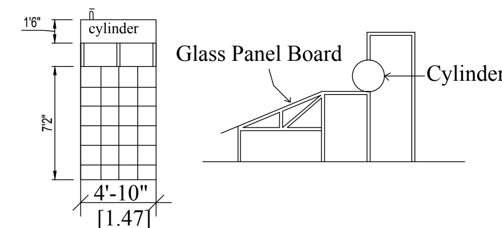
SOLAR ENERGY SYSTEM
