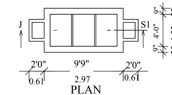
'I' type trap 2 Nos in inlet, outlet & Vent pipe will be covered with to proof covering net in inner side and top of vent pipe.
