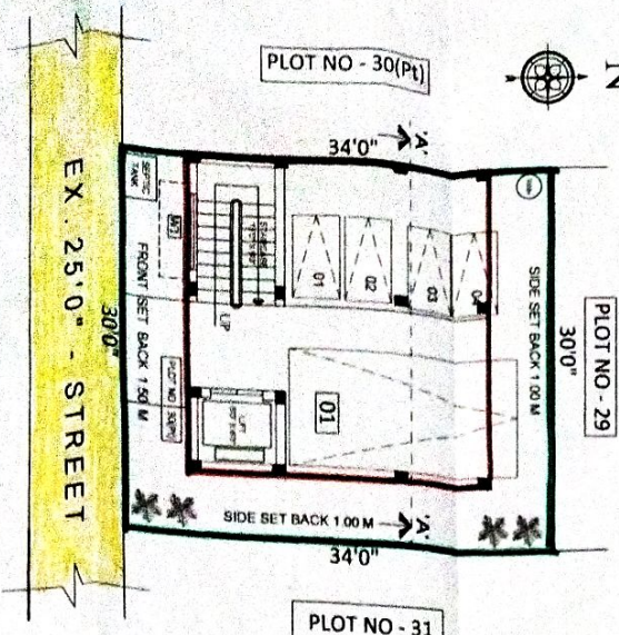
STILL - CUM SITE FLOOR PLAN
