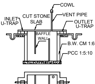
SEPTIC TANK DETAILS SIZE :6'0" x 3'0" x 6'0"
