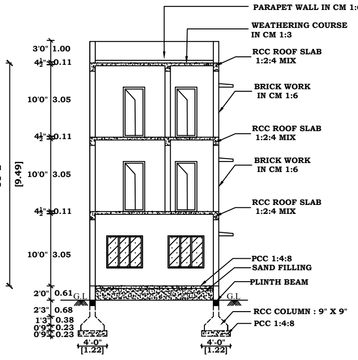
SECTION - KK
