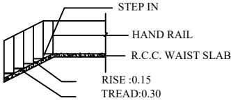
STAIR DETAILS
