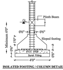
ISOLATED FOOTING / COLUMN DETAIL
