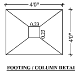
FOOTING / COLUMN DETAIL
