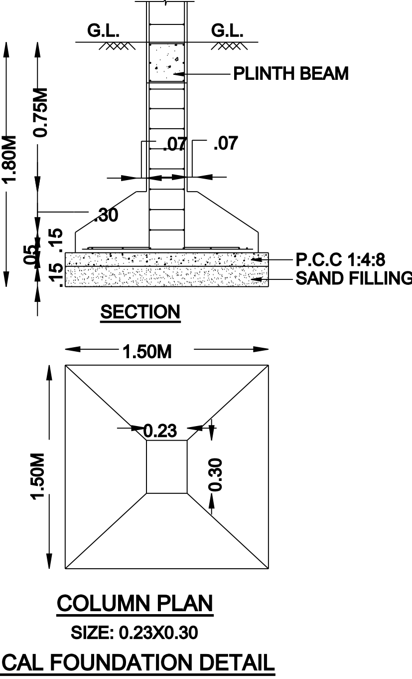
TYPICAL FOUNDATION DETAIL
