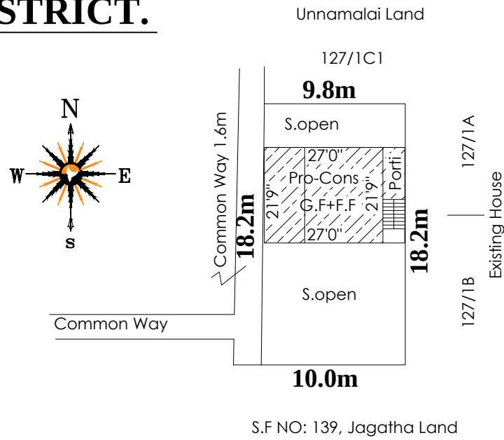
SITE PLAN SCALE: 1 INCH = 33 FEET
