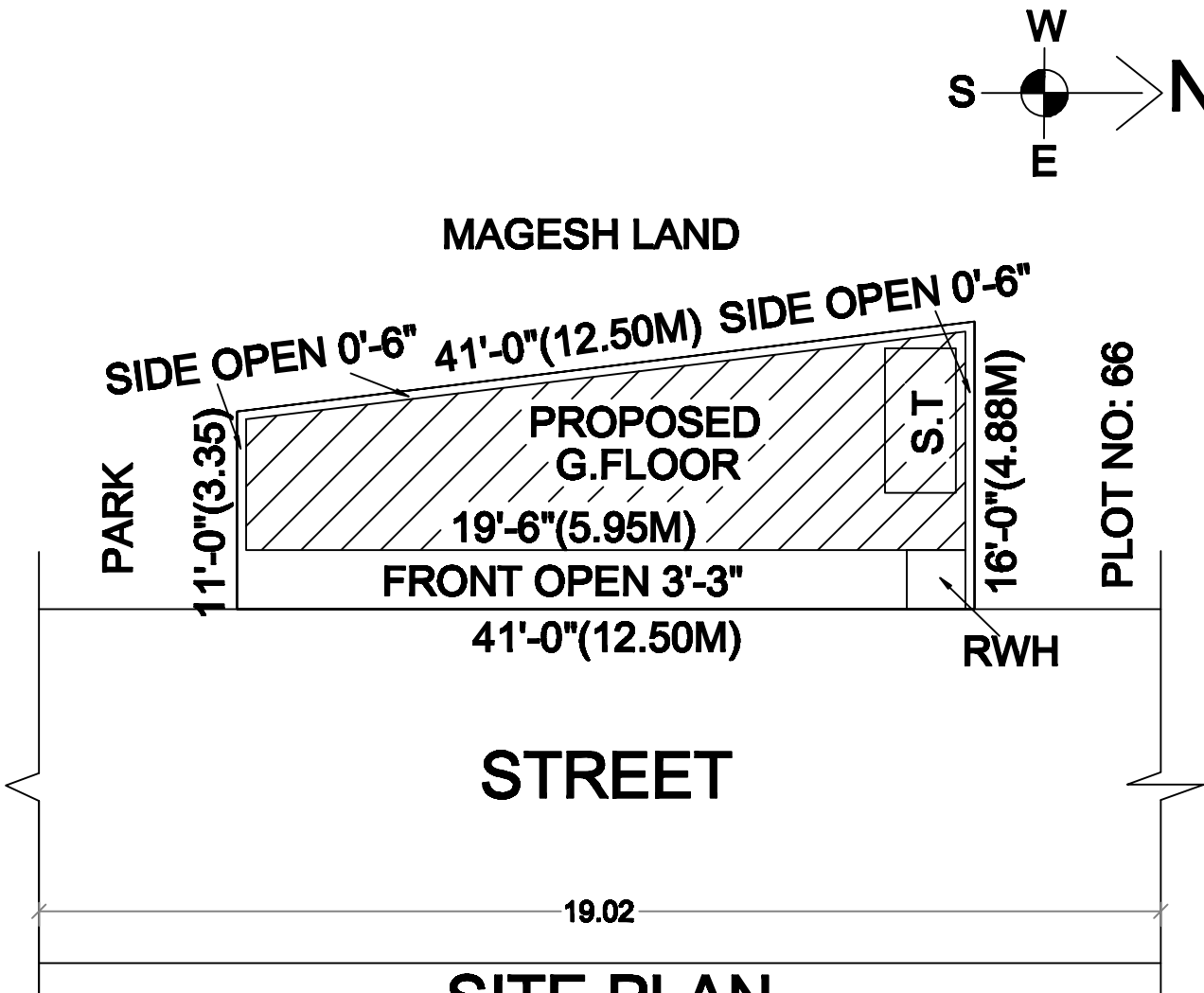
SITE PLAN (SCALE: 1CM : 1M)
